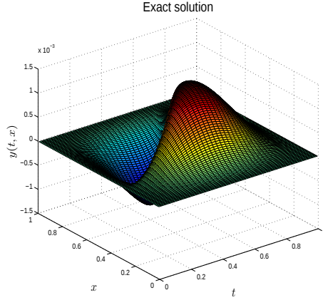
FIG. 5.1. Exact solution of the semilinear parabolic PDE.
