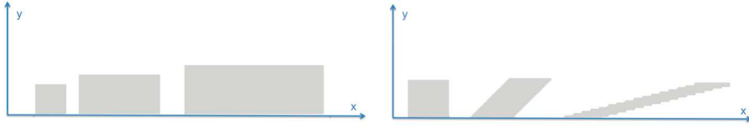
Figure 1.2: Effect of parabolic scaling and shearing on square region. left: Parabolic scaling causes the region evolve along one axis more than the other one. Therefore regions loses its characteristic and become more elongated. right: Shearing operator shifts the upper vertices of square along a line parallel to x-axis. This causes very thin regions in large shearing factors.
