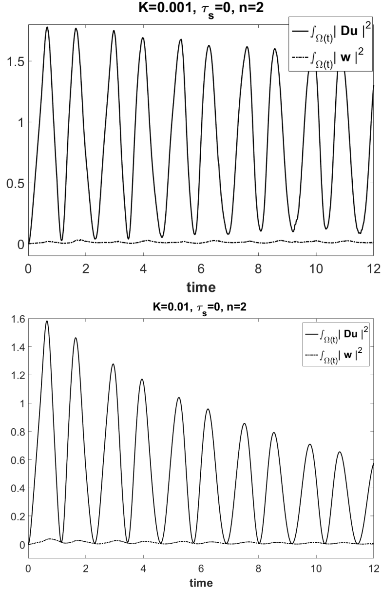
Figure 3.2: The evolution of \int_{\Omega(t)} |\mathbf{Du}|^2 d\mathbf{x} and of the enstrophy, \int_{\Omega(t)} |\mathbf{w}|^2 d\mathbf{x} , with \mathbf{w} = \frac{1}{\sqrt{2}} \nabla \times \mathbf{u} . All results are computed for n = 2 .
