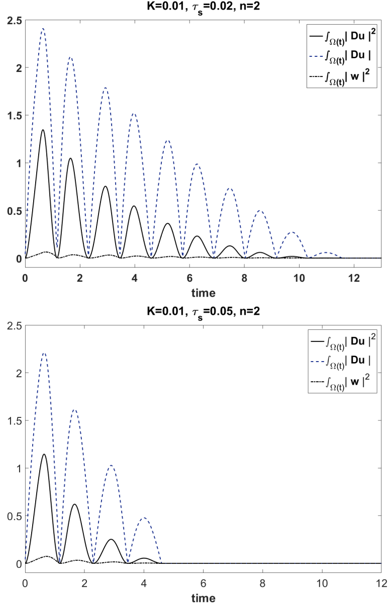
Figure 4.1: The evolution of \int_{\Omega(t)} |\mathbf{Du}|^2 d\mathbf{x} and of the enstrophy, \int_{\Omega(t)} |\mathbf{w}|^2 d\mathbf{x} , with \mathbf{w} = \frac{1}{\sqrt{2}} \nabla \times \mathbf{u} . All results are computed for n = 2 and different values of \tau_s . For \tau_s > 0 the figure also shows \int_{\Omega(t)} |\mathbf{Du}| d\mathbf{x} .
