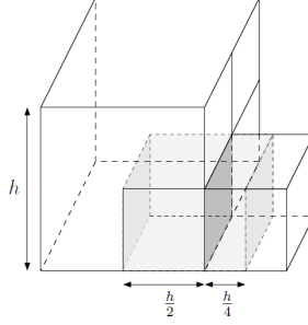
Figure 2.4: Reference points for the diffusion flux approximation
