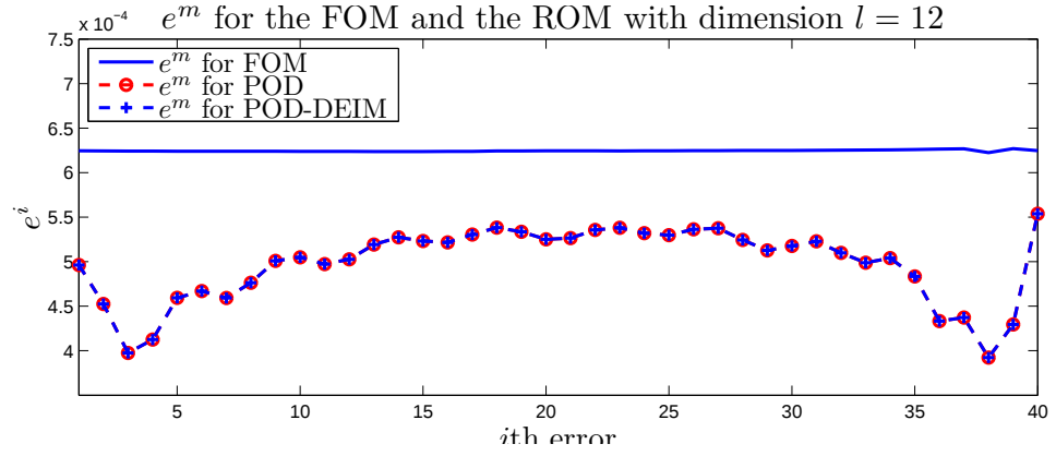
Figure 5.25: Example 3: Error estimators e^m and e_{rom}^m for the ROM with dimension l = 12
