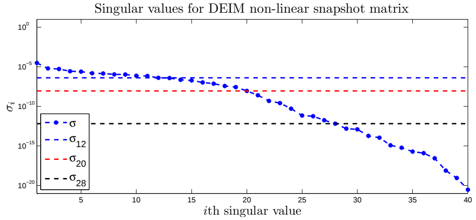
Figure 5.14: Example 2: Singular values \{\sigma_i\}_{i=1}^{40} for DEIM non-linear snapshot matrix.
