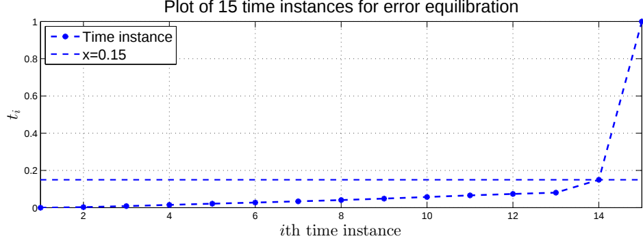
Figure 5.9: Example 1: 15 time instances for the error equilibration for FOM .
