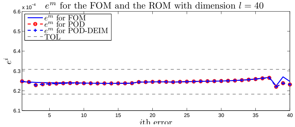
Figure 5.28: Example 3: Error estimators e^m and e_{rom}^m for the ROM with dimension l = 40
