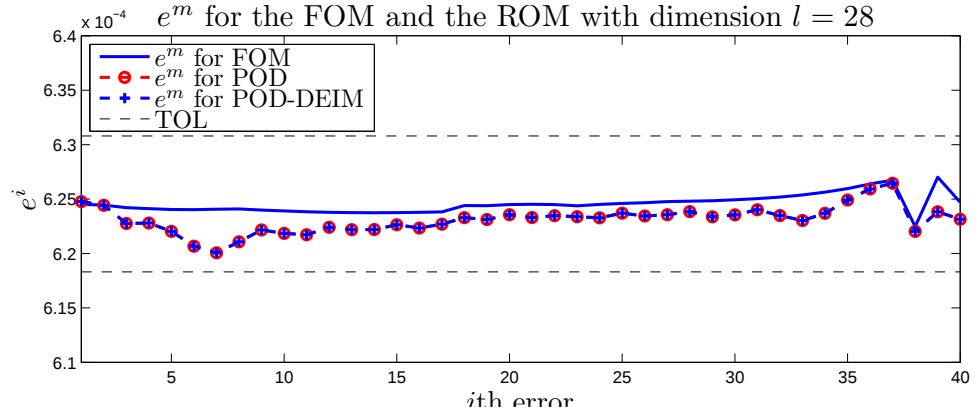
Figure 5.27: Example 3: Error estimators e^m and e_{rom}^m for the ROM with dimension l = 28
