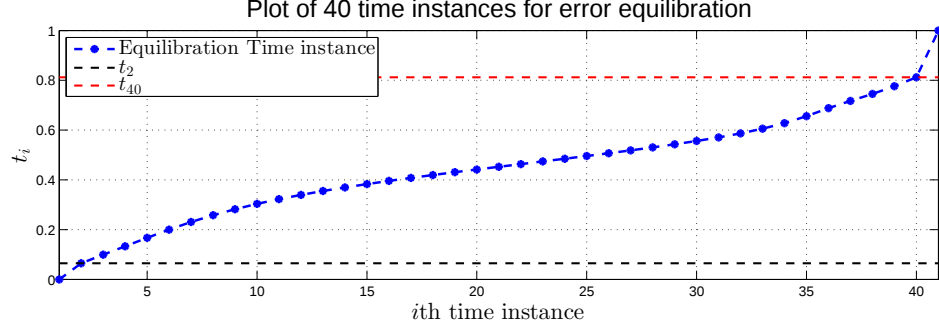
Figure 5.12: Example 2: 40 time instances for error equilibration for non-linear FOM .
