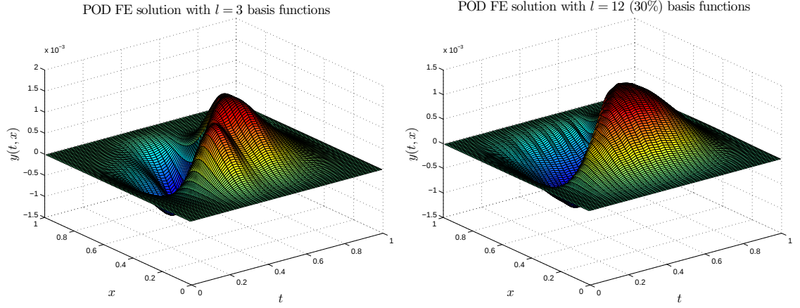
Figure 5.15: Example 2: Implicit Euler FE solution for POD based ROM with dimension l = 3 (Left), 12 (Right).
