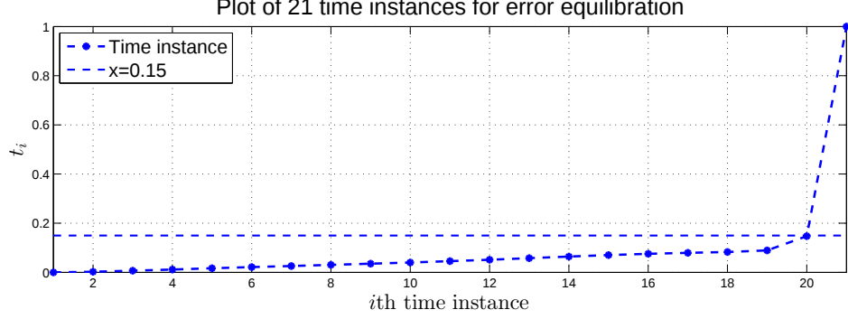
Figure 5.2: Example 1: 21 time instances for the error equilibration for FOM
