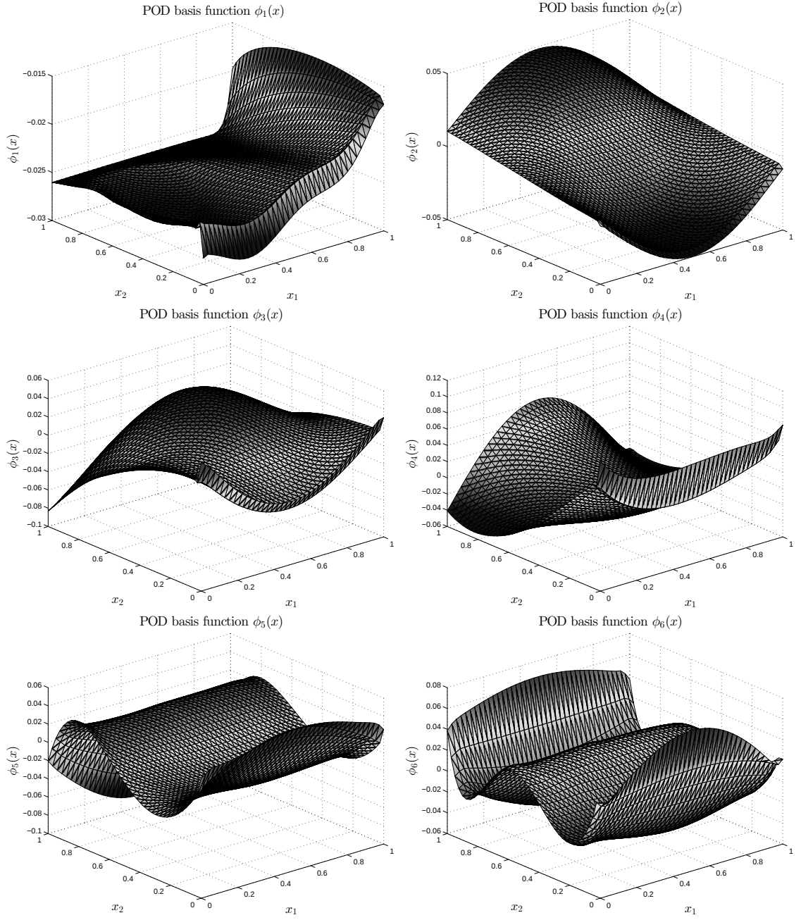
Figure 5.4: Example 1: The first 6 POD basis functions
