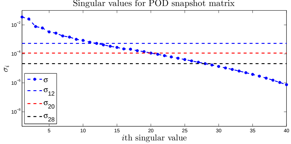
Figure 5.23: Example 3: Singular values \{\sigma_i\}_{i=1}^{40} for POD snapshot matrix.
