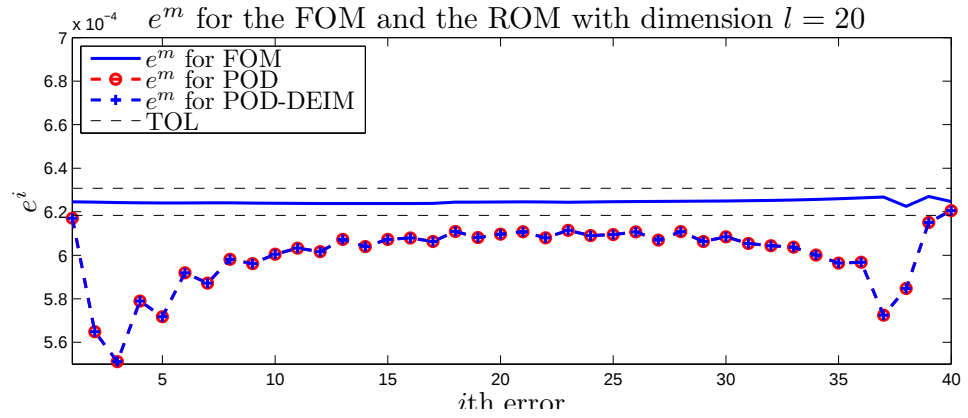
Figure 5.26: Example 3: Error estimators e^m and e_{rom}^m for the ROM with dimension l = 20
