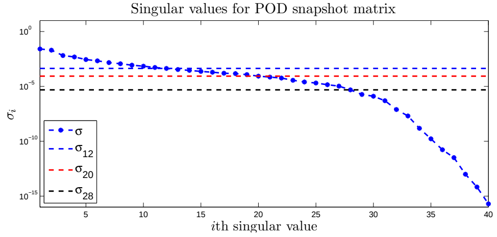
Figure 5.13: Example 2: Singular values \{\sigma_i\}_{i=1}^{40} for POD snapshot matrix.
