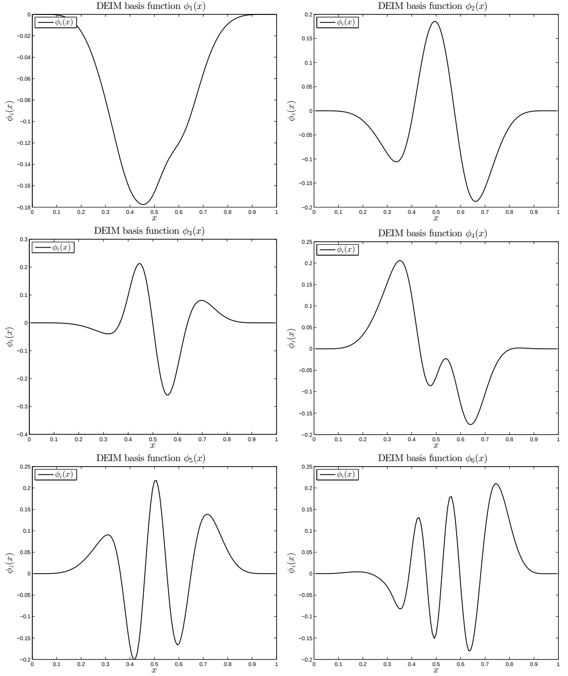
Figure 5.18: Example 2: Plot of the first 6 basis functions for DEIM
