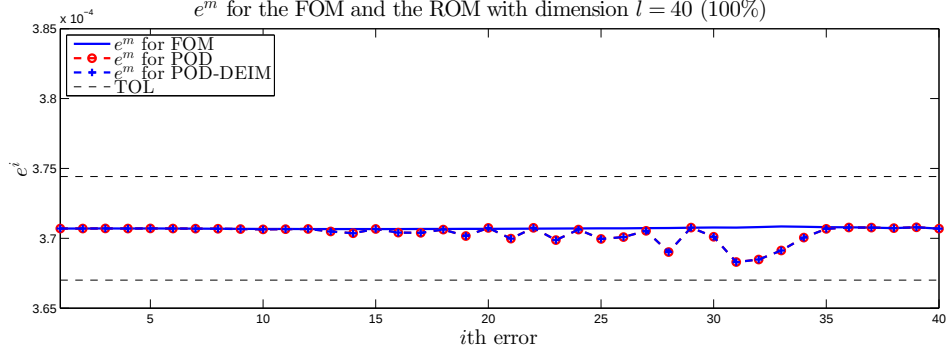
Figure 5.22: Example 2: Error estimators e^m and e_{rom}^m for the ROM with dimension l = 40
