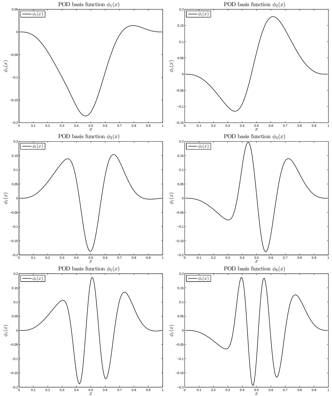
Figure 5.17: Example 2: Plot of the first 6 POD basis functions
