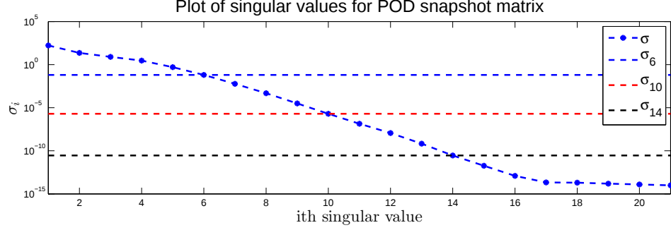
Figure 5.3: Example 1: Singular values \{\sigma_i\}_{i=1}^{21} for the POD snapshot matrix.
