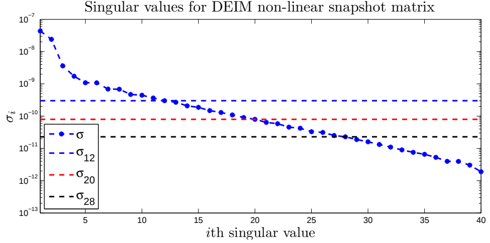
Figure 5.24: Example 3: Singular values \{\sigma_i\}_{i=1}^{40} for DEIM non-linear snapshot matrix.
