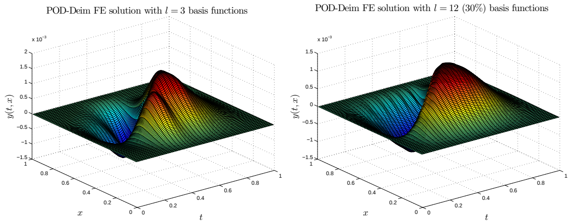
Figure 5.16: Example 2: Implicit Euler FE solution for POD-DEIM based ROM with dimension l = 3 (Left), 12 (Right).
