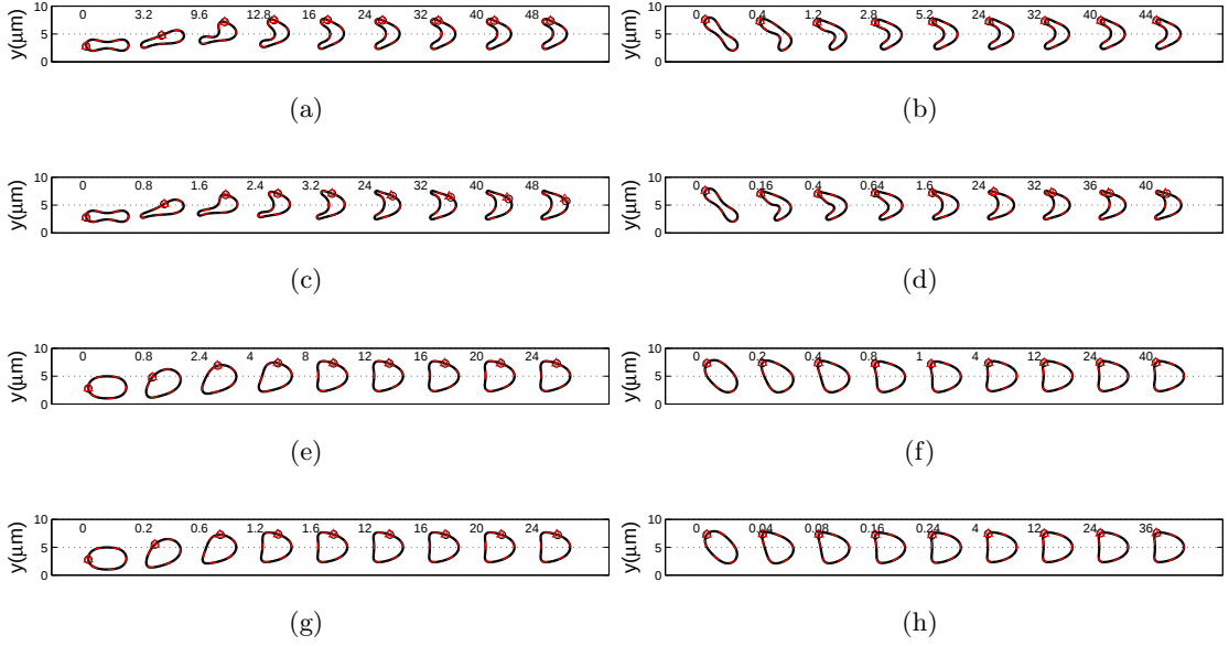
Figure 3.9: The snapshots of motions of RBC under two different flow models with bending constant 0.1k_b . The cell swelling ratio is 0.481 in the upper four plots and 0.9 in the lower four plots. The capillary number are 0.65 and 3.27 for the plots in row one,three and two,four respectively. the circle, triangle denotes the same mark on the cell membrane.
