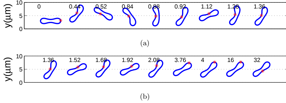
Figure 3.18: The snapshots of motions of a stiff biconcave RBC in Poiseuille flow. The number above each snapshot marks the time in millisecond (ms).
