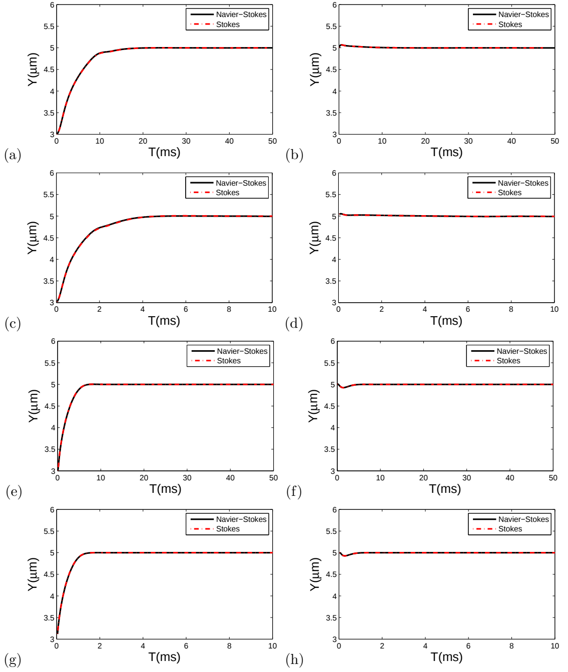
Figure 3.7: The trajectory of cell mass center with cell bending constant 0.1k_b . The swelling ratio is 0.481 (a,b,c,d) and 0.9 (e,f,g,h) and the capillary number is 0.65 (a,b,e,f) and 3.27 (c,d,g,h), respectively.
