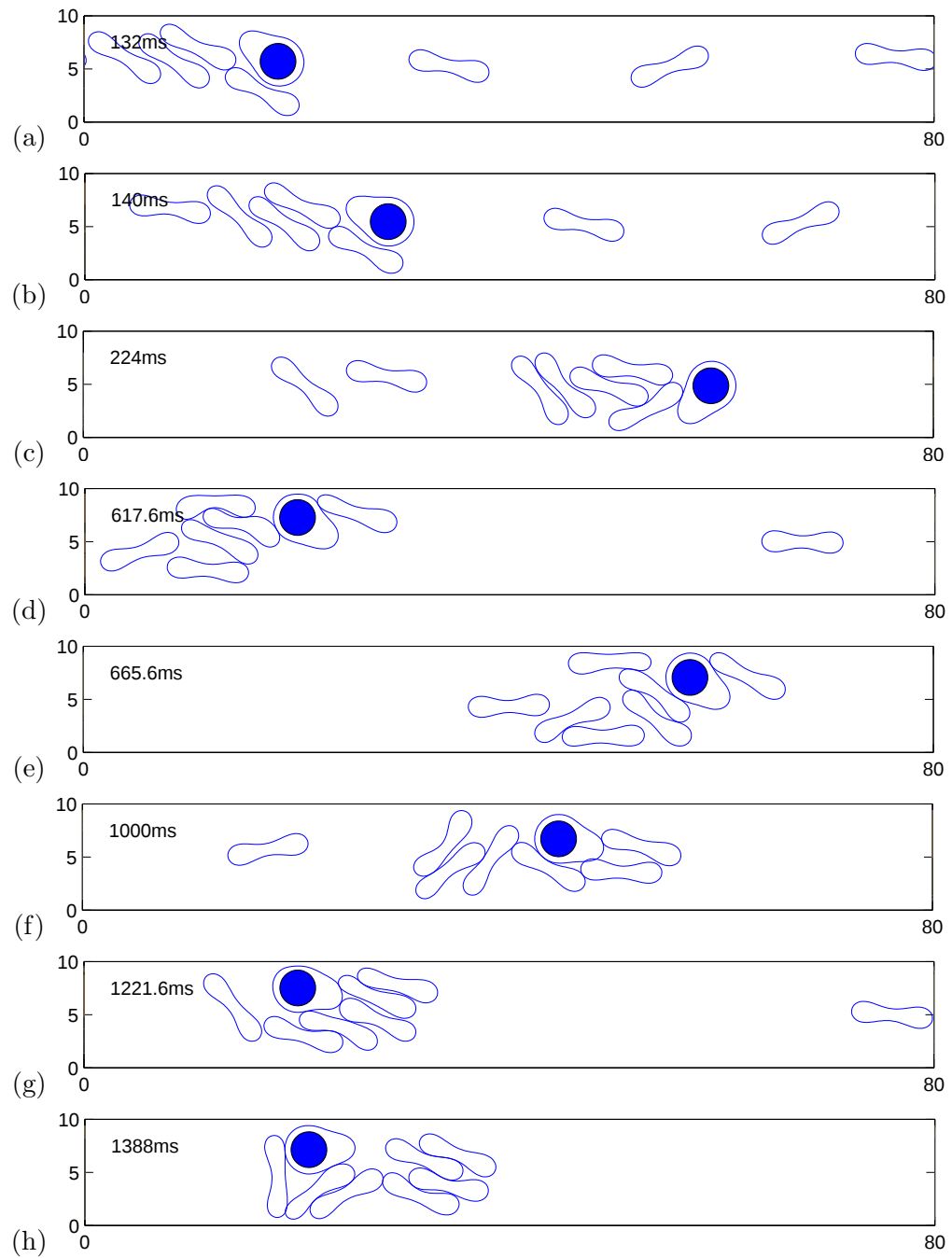
Figure 4.10: More snapshots of interaction between 7 healthy RBCs and a sick iRBC.
