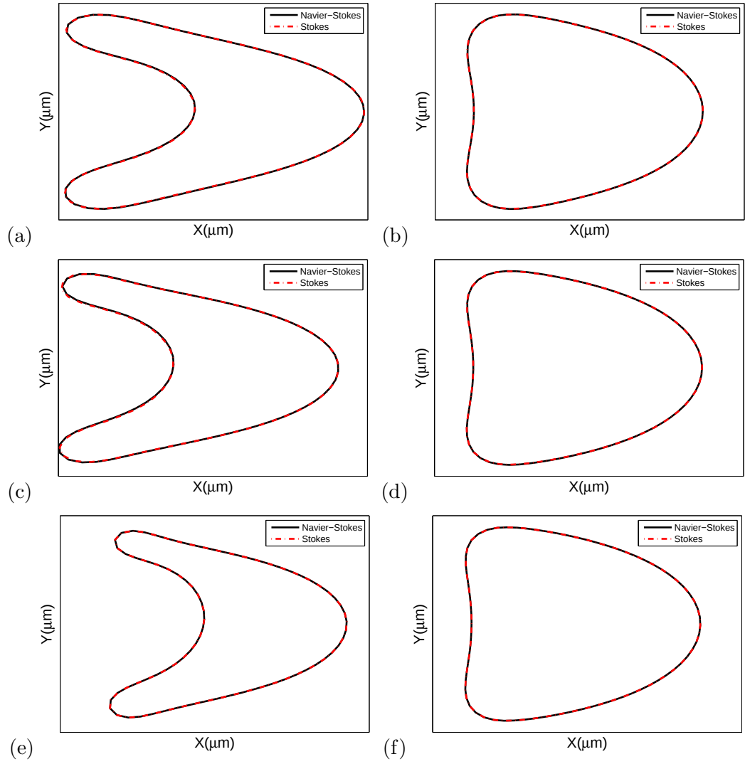
Figure 3.14: Final shapes of RBCs with cell swelling ratio s^* = 0.481 (a,c,e) and 0.9 (b,d,f). The maximum flow speeds are u_{max} = 18, 36 , and 54 cm/s for the top, middle and bottom rows, respectively. Bending constant is 1k_b .
