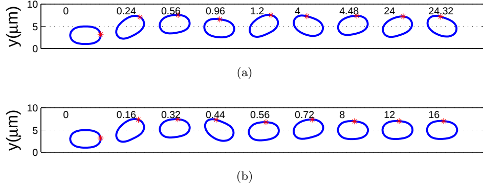
Figure 3.19: The snaking motion in NS flow and the damped oscillation motion in Stokes flow of an elliptical cell. The bending is 100k_b , the speed at the center line of the flow is 54\text{cm/s} . The number above each snapshot marks the time in millisecond (ms).
