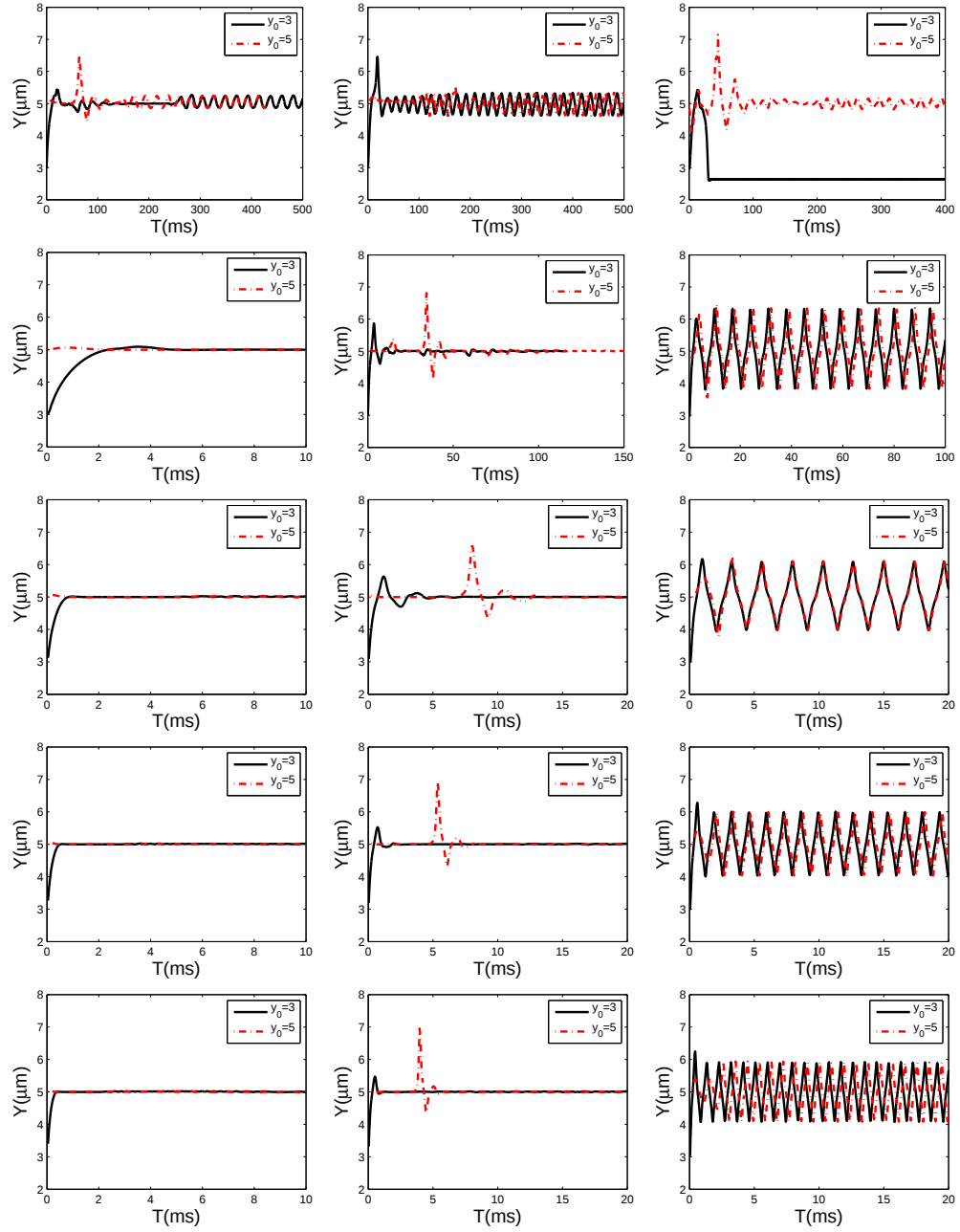
Figure 4.4: History of trajectory of cell mass center. The filling fraction is \Phi = 0.2, 0.3, 0.4 from left to right for each row. The velocity at centerline is u_{max} = 1, 5, 15, 25, 35 cm/s from up to low.
