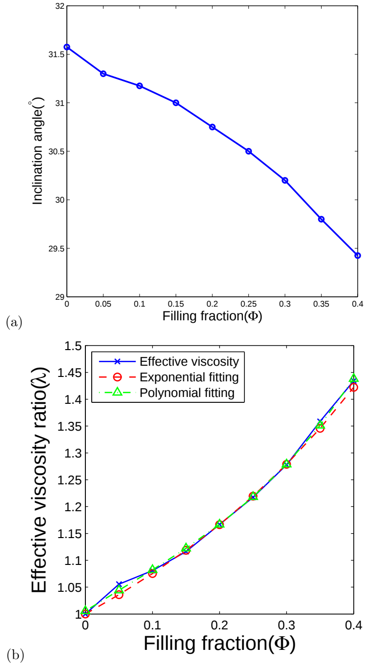
Figure 5.4: Equilibrium inclination angle of compound iRBC with inclusion ratio \Phi = 0.05, 0.1, 0.15, 0.2, 0.25, 0.3, 0.35, 0.4 and corresponding effective viscosity ratio.
