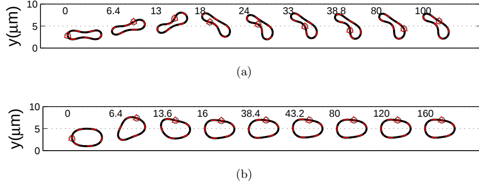
Figure 3.11: The snapshots of damped oscillations of RBC under two different flow models with bending constant 1k_b in flow. The circle, asterisk denotes the same mark on the cell membrane.
