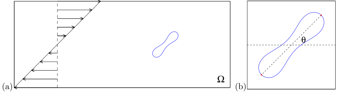
Figure 5.1: An schematic diagram of a single red blood cell in shear flow with the computational domain \Omega , the inclination angle \theta is defined as the angle between the cell long axis and the horizontal line.
