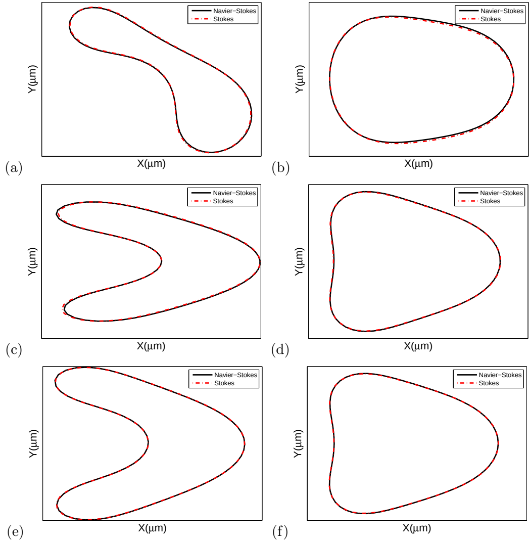
Figure 3.15: Final shapes of RBCs with cell swelling ratio s^* = 0.481 (a,c,e) and 0.9 (b,d,f). The maximum flow speeds are u_{max} = 18, 36 , and 54 cm/s for the top, middle and bottom rows, respectively. Bending constant is 10k_b .
