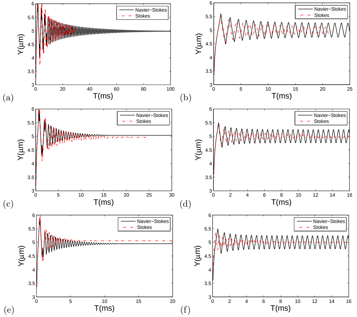
Figure 3.16: Trajectory of cell mass center with cell swelling ratio s^* = 0.481 (a,c,e) and 0.9 (b,d,f). The maximum flow speed is u_{max} = 18, 36 , and 54 cm/s for three rows, respectively. Bending constant is 100k_b .
