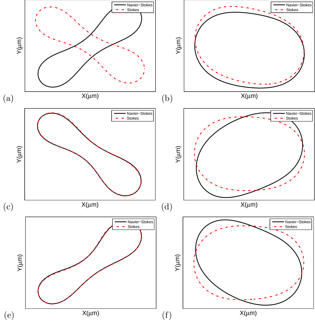
Figure 3.17: Final shapes of RBCs with cell swelling ratio s^* = 0.481 (a,c,e) and 0.9 (b,d,f). The maximum flow speed is u_{max} = 18, 36 , and 54 cm/s for three rows, respectively. Bending constant is 100k_b .
