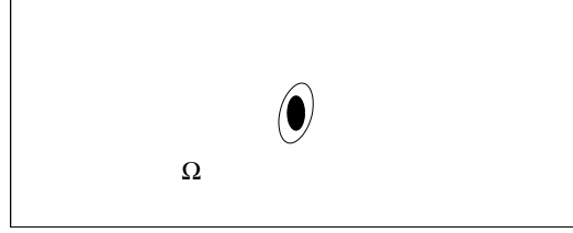
Figure 2.3: An example of computational domain with one malaria-infected RBC.
