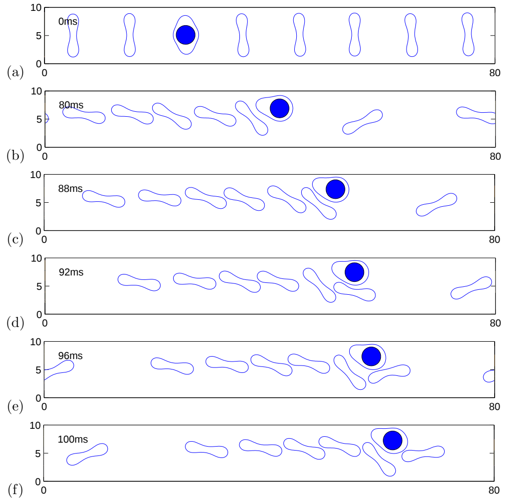
Figure 4.9: Snapshots of interaction between 7 healthy RBCs and a sick iRBC.
