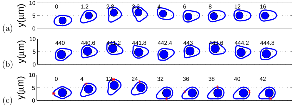
Figure 4.3: Snapshots of motions of iRBC in channel flow. The snapshot (a) is of iRBC with \Phi = 0.3 , y_0 = 5\mu\text{m} and u_{max} = 5\text{cm/s} , the cell stays at the center of the flow. The snapshot (b) is of iRBC with \Phi = 0.4 , y_0 = 5\mu\text{m} and u_{max} = 15\text{cm/s} , the cell keeps oscillating up and down. The snapshot (c) is of iRBC with \Phi = 0.4 , y_0 = 3\mu\text{m} and u_{max} = 1\text{cm/s} , the cell is pushed to the side of the channel and undergoes a tank-treading motion. The red asterisk marks the trajectory of the same point on the mambrane of an iRBC. The number above each snapshot marks the time in millisecond (ms).
