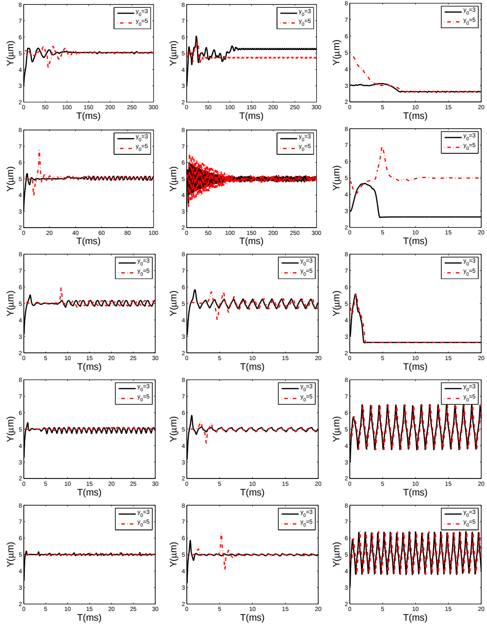
Figure 4.5: History of trajectory of cell mass center. The filling fraction is \Phi = 0.2, 0.3, 0.4 from left to right for each row. The velocity at centerline is u_{max} = 1, 5, 15, 25, 35 \text{ cm/s} from up to low.
