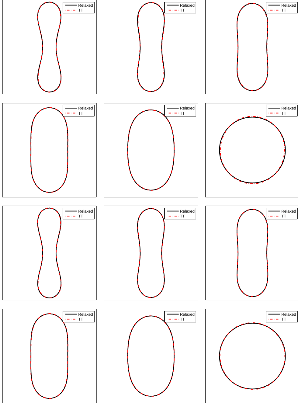
Figure 3.2: Comparison between relaxed cell shapes and tank-treading shapes of RBCs with swelling ratio s^* = 0.481, 0.6, 0.7, 0.8, 0.9, 1.0 . Degrees of confinement is 0.4 for the upper two rows and 0.8 for the lower two rows.
