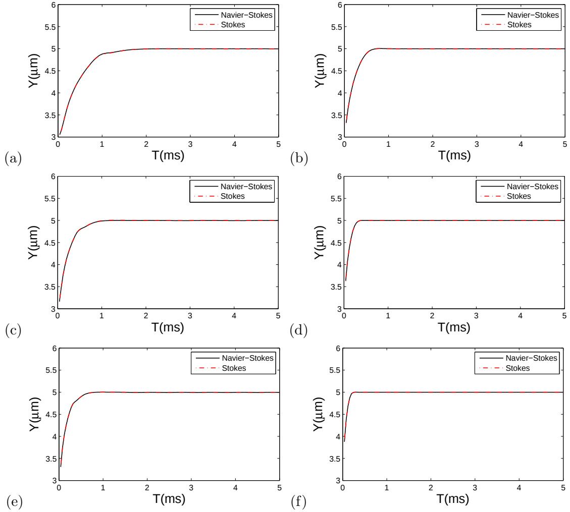
Figure 3.12: Trajectory of cell mass center with cell swelling ratio s^* = 0.481 (a,c,e) and 0.9 (b,d,f). The maximum flow speed is u_{max} = 18, 36 , and 54 \text{ cm/s} for three rows, respectively. Bending constant is 1k_b .
