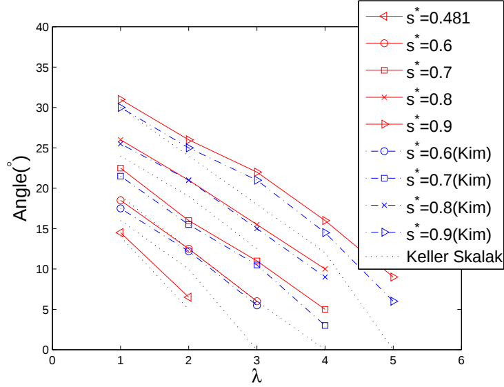
Figure 5.3: Steady inclination angle \theta as a function of the viscosity ratio \lambda for different values of the swelling ratio s^* .
