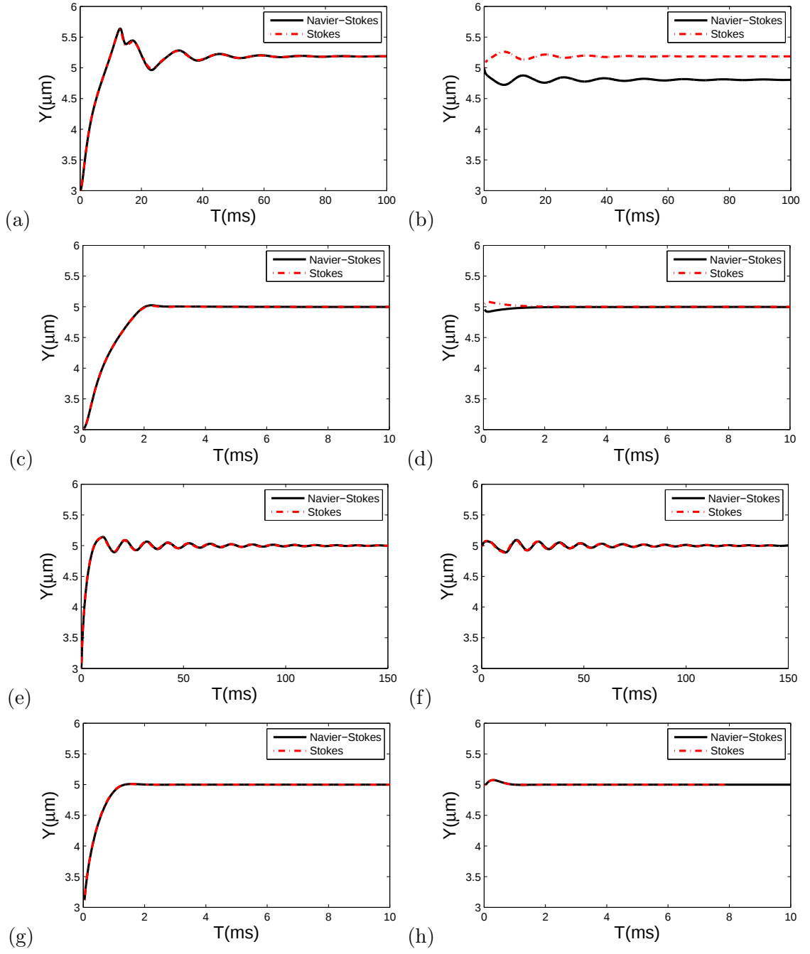
Figure 3.8: The trajectory of cell mass center with cell bending constant 1k_b . The swelling ratio is 0.481 (a,b,c,d) and 0.9(e,f,g,h) and the capillary number is 0.065 (a,b,e,f) and 0.327 (c,d,g,h), respectively.
