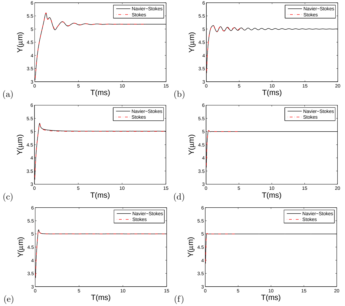
Figure 3.13: Trajectory of cell mass center with cell swelling ratio s^* = 0.481 (a,c,e) and 0.9 (b,d,f). The maximum flow speed is u_{max} = 18, 36 , and 54 cm/s for three rows, respectively. Bending constant is 10k_b .
