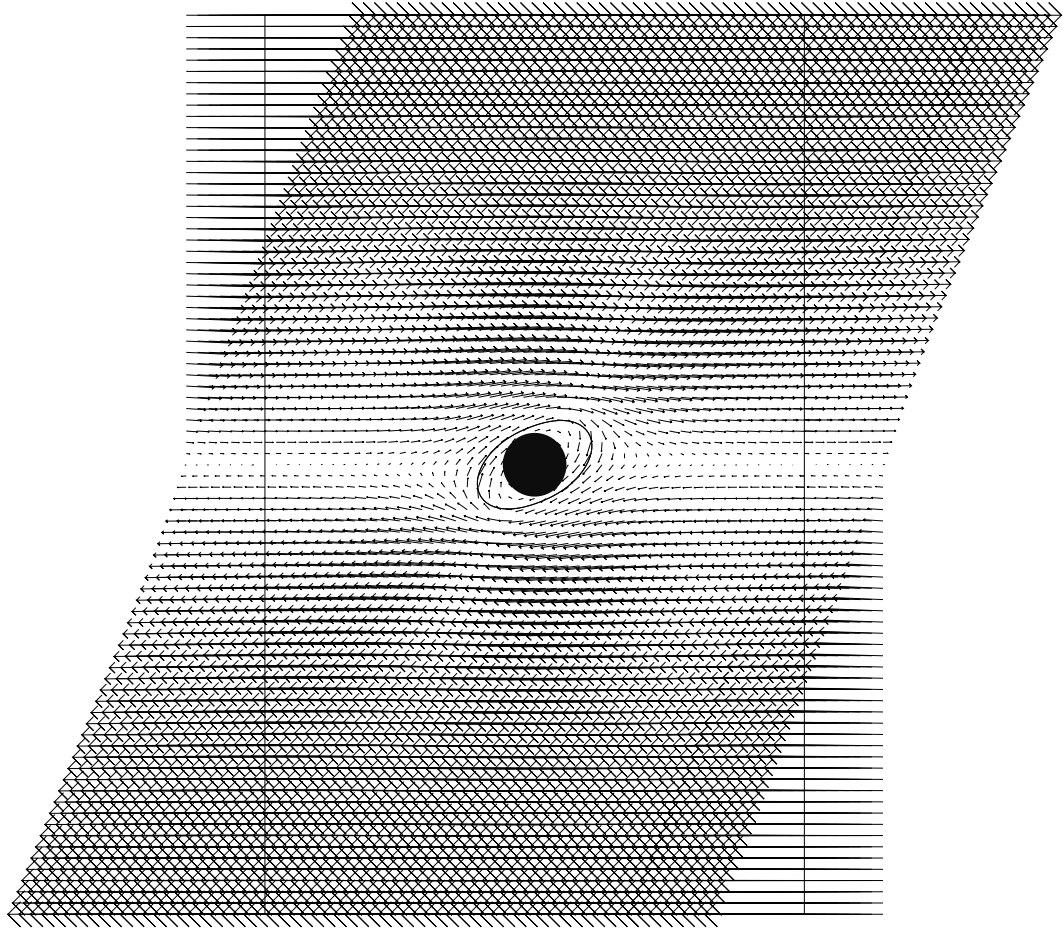
Figure 5.6: Velocity field of a compound iRBC tank-treading in a shearflow in a domain of 30 \times 50 \mu\text{m}^2 .
