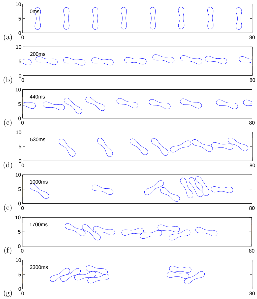
Figure 4.7: Snapshots of 8 healthy RBC in channel flow.
