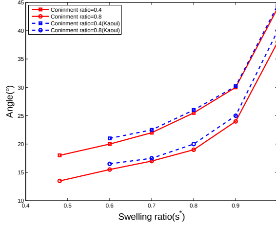
Figure 3.4: Steady inclination angle as a function of the cell swelling ratio for two degrees of confinement R_0/w=0.4 and 0.8 .
