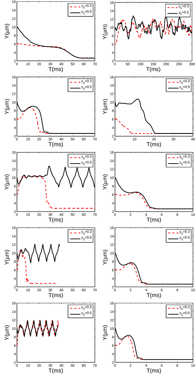
Figure 4.6: History of trajectory of cell mass center in a wide channel with same Reynolds number as in the narrow channel. The left column is iRBC with 1k_B and 10k_b on the right.
