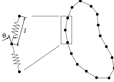
Figure 2.2: The elastic spring model of the RBC membrane
