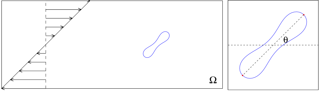
Figure 3.1: An schematic diagram of a single red blood cell in shear flow with the computational domain \Omega , the inclination angle \theta is defined as the angle between the cell long axis and the horizontal line.
