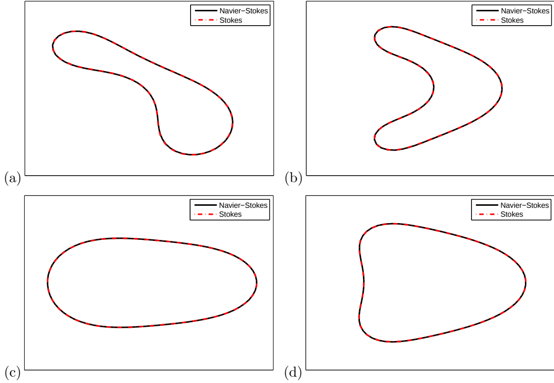
Figure 3.6: The final equilibrium shape of RBCs with 1k_b in bounded Poiseuille flow. Cell swelling ratio is s^* = 0.481 (a,b) and 0.9 (c,d) , and the flow capillary number Ca = 0.065 (a,c) and 0.33 (b,d), respectively.
