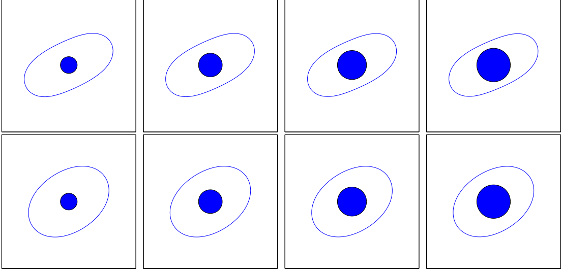
Figure 4.1: Final steady tank treading state of a compound iRBC in shear flow. The filling fraction is \Phi = 0.05, 0.10, 0.15, 0.20 from left to right for each row. The cell swelling ratio is 0.84 for the upper row and 0.95 for the lower row.
