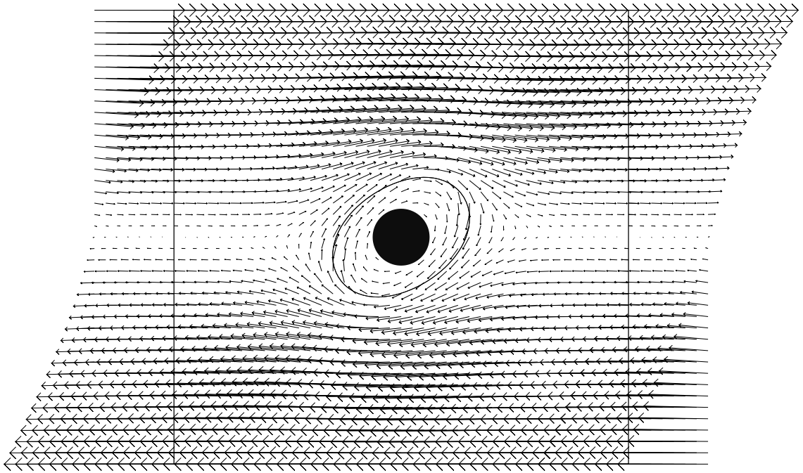
Figure 5.5: Velocity field of a compound iRBC tank-treading in a shearflow in a domain of 20 \times 20 \mu\text{m}^2 .
