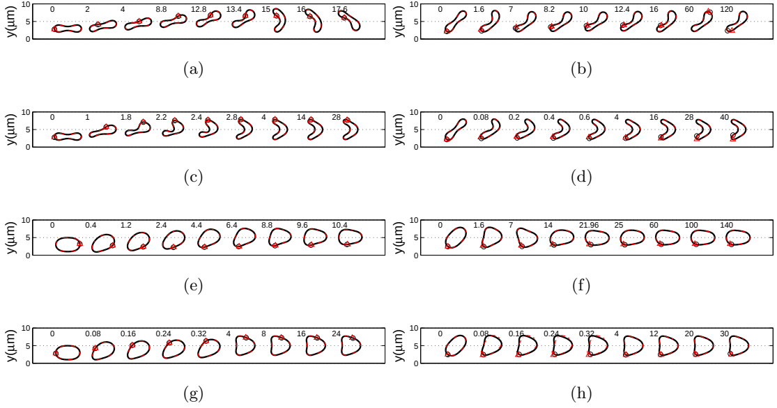
Figure 3.10: The snapshots of motions of RBC under two different flow models with bending constant 1k_b . The cell swelling ratio is 0.481 in the upper four plots and 0.9 in the lower four plots. The capillary number are 0.065 and 0.327 for the plots in row one,three and two,four respectively. the circle, asterisk denotes the same mark on the cell membrane.
