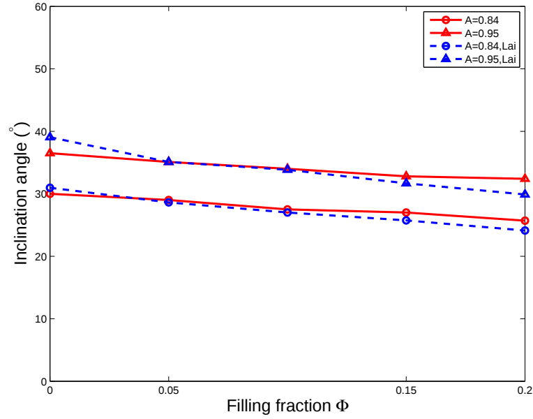
Figure 4.2: Plot of steady inclination angle as a function of filling fraction.
