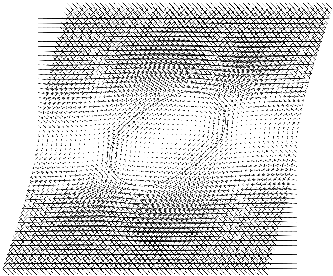
Figure 5.7: Velocity field of the inner circulation in a RBC.
