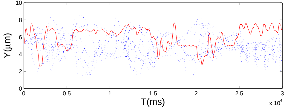
Figure 4.11: Trajectory of the cell mass centers in channel flow.
