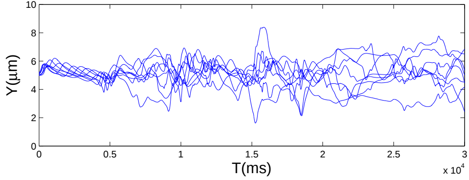
Figure 4.8: Trajectory of the cell mass centers in channel flow.
