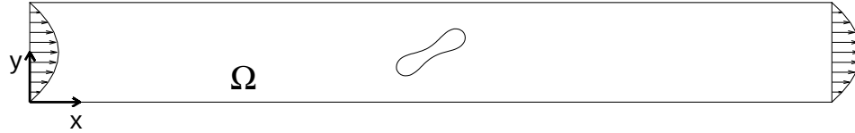
Figure 2.1: Schematic of a single red blood cell in plane Poiseuille flow with the computational domain \Omega .
